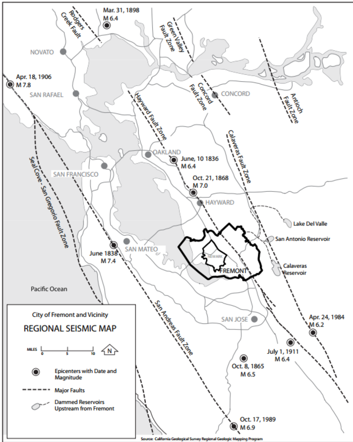
Map 10 – Regional Seismic Activity Map
